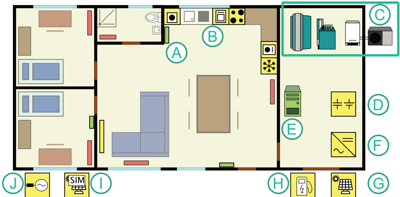
Ground Plan of the 60m 2 flat with intelligent household appliances and controllable electrical equipment, A: Energy Management Panel; B: Intelligent electrical devices; C: Heating System: Warm water storage, el. heating rod, micro-CHP, heat pump; D: Hybrid battery system; E: Energy Management System; F: Solar power inverter; G: PV system; H: EV charging point; I: PV simulator; J: Artificial mains network
